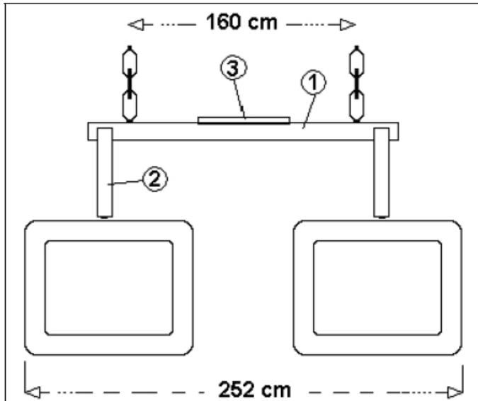
Fig. 17: New Look 28" monitors hung in the center of the lane. The horizontal bar (1) MEC-Y-MW0053C has a shelf to support the lane computer (3), The monitors are hung using the vertical bars (2). The entire structure is hung using chains. It is possible to hang WinVision28" monitors with this same mechanism. Without the center panel usually used with this monitor style.
