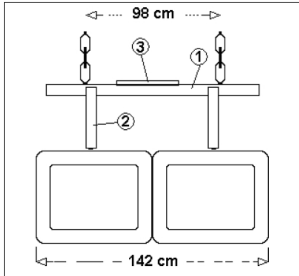
Fig. 18: New Look 28" monitors hung next to one another. The horizontal bar (1) MEC-Y-MW0053C has a shelf to support the lane computer (3), the monitors are hung using the vertical bars (2) The entire structure is hung using chains.
